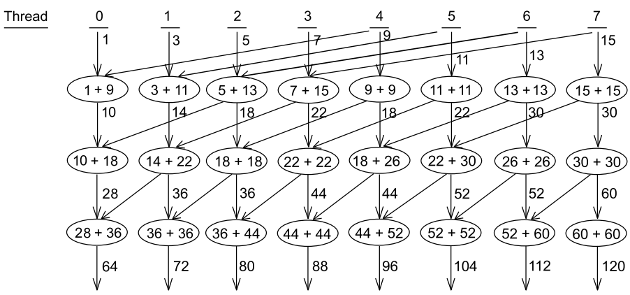
FIGURE 6.5 Tree-structured sum using warp shuffle.
